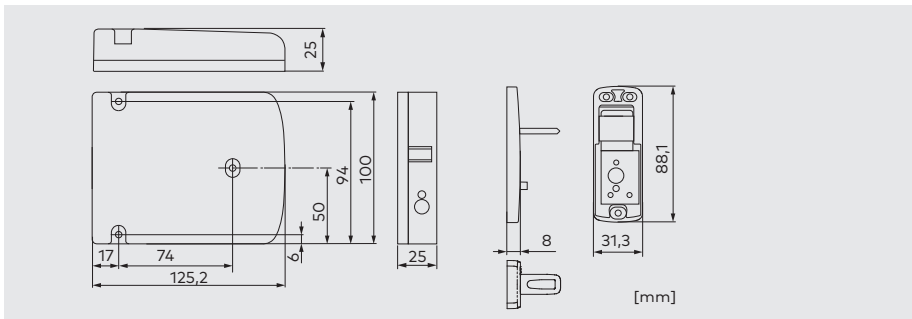
cabinet lock 21 10: side lock with door latch for non-metal doors
